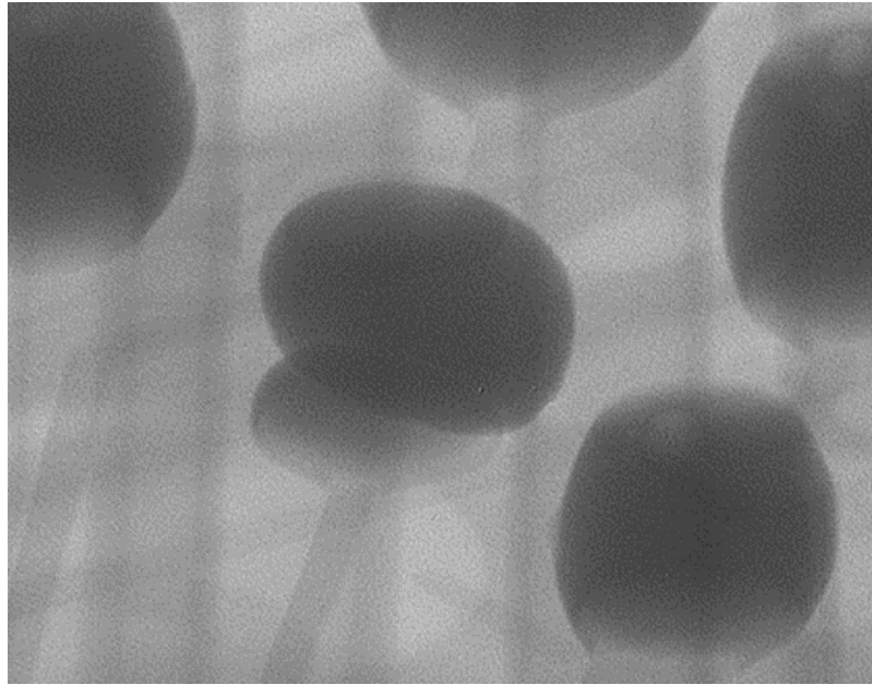
Head-on-pillow
